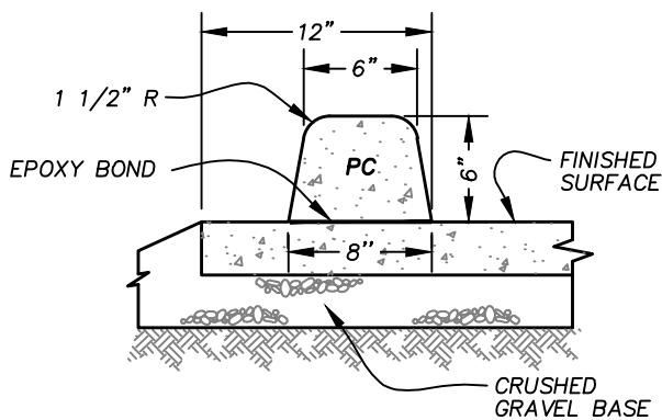
EXTRUDED PC CONCRETE BONDED CURB
