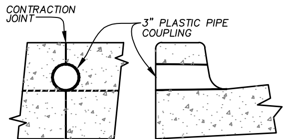
WEEP HOLE THROUGH CURB
