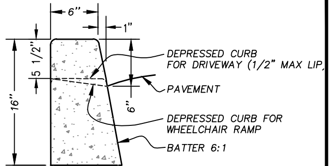
TYPICAL VERTICAL (STRAIGHT) CURB
