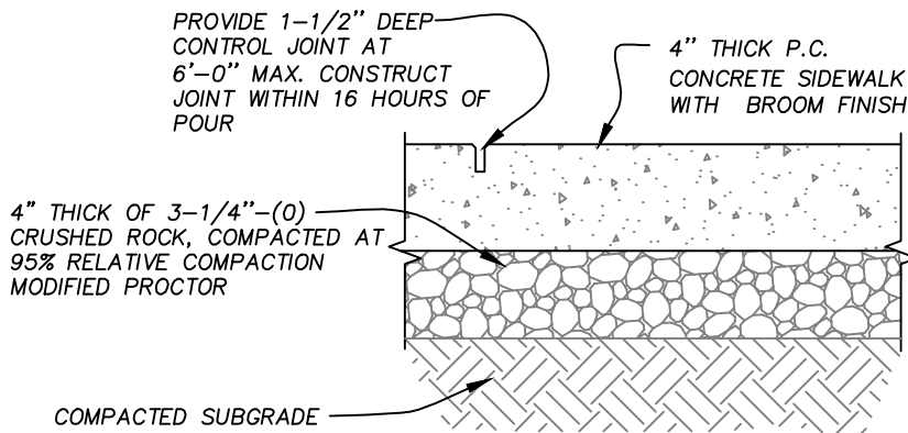
SIDEWALK PAVING SECTION
